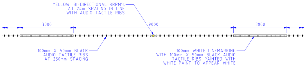
Figure B.1.1 – Two-Way Dividing ATCL
