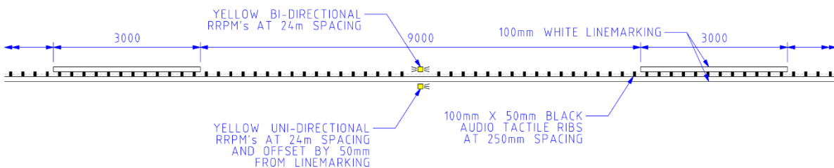
Figure B.1.4 – Double One-Way Barrier ATCL
