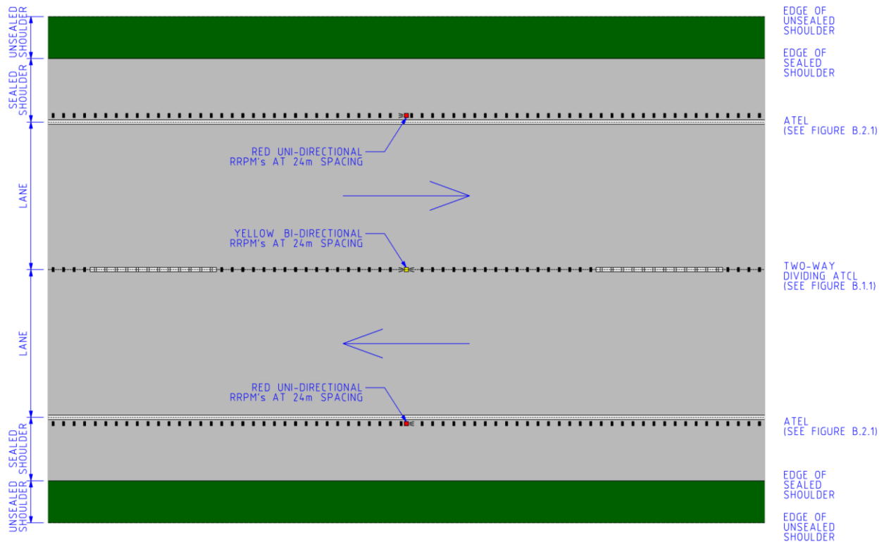
Figure C.2.1 – Plan Layout with Two-Way Dividing ATCL and Audio Tactile Edge Line (ATEL)
