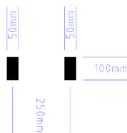
Figure 5.0.1 Audio tactile ribs dimensions and spacing
