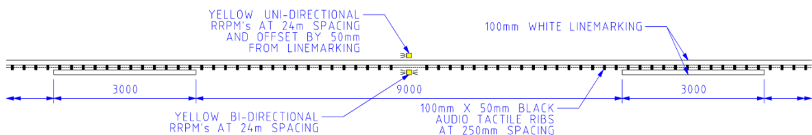
Figure B.1.5 – Double One-Way (Reverse) Barrier ATCL
