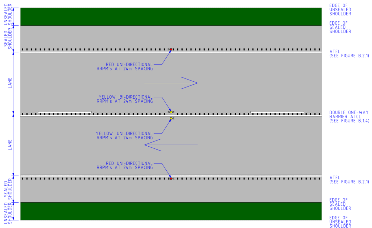
Figure C.2.3 – Plan Layout with Double One-Way Barrier ATCL and Audio Tactile Edge Line (ATEL)
