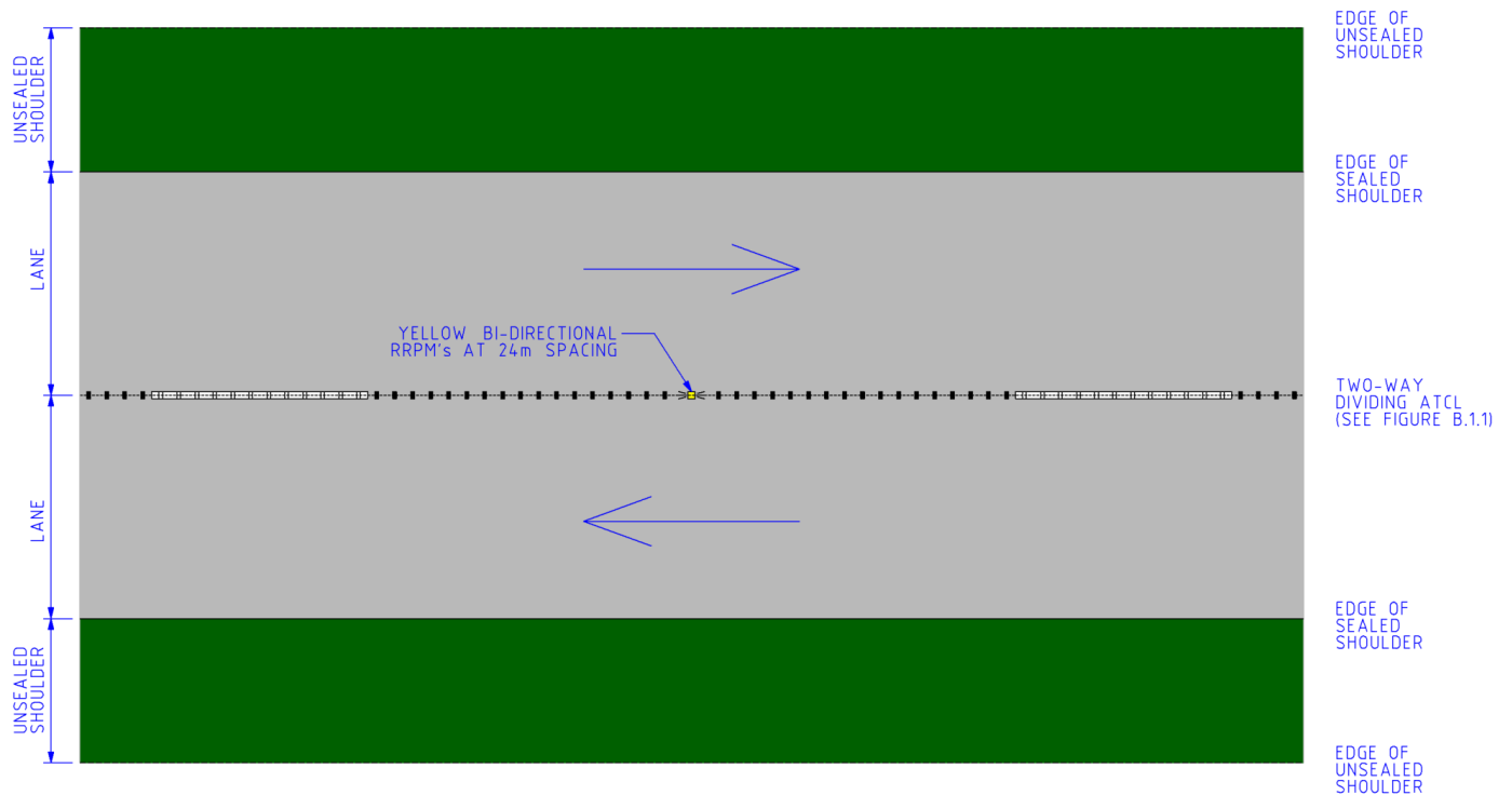
Figure C.1.1 – Plan Layout for Narrow Sealed Roads with Two-Way Dividing ATCL
