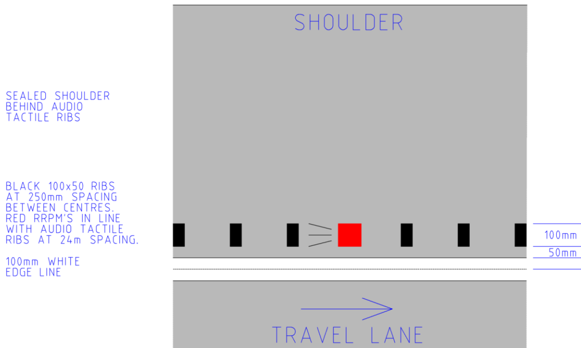
Figure B.2.1 – Standard ATEL
