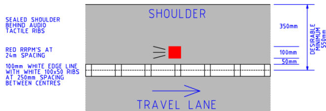
Figure 5.2.1.3 Retrofit ATEL Installation - Desirable minimum sealed shoulder 0.55m with on-line audio tactile ribs
