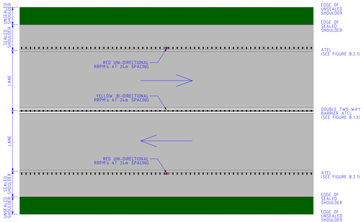
Figure C.2.2 – Plan Layout with Double Two-Way Barrier ATCL and Audio Tactile Edge Line (ATEL)
