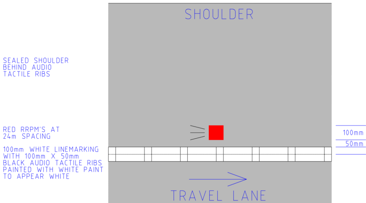
Figure B.2.2 – On-line ATEL (for areas of minimum seal width)
