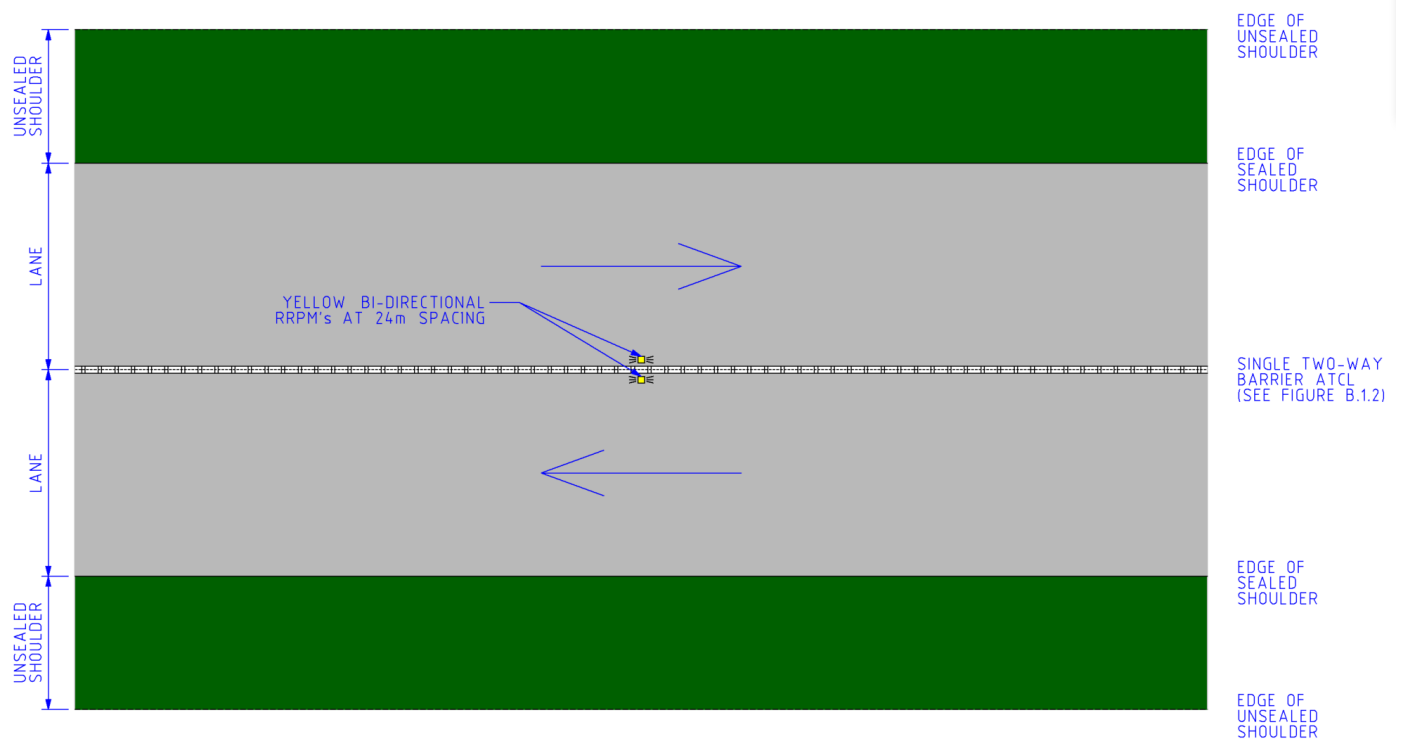
Figure C.1.2 – Plan Layout for Narrow Sealed Roads with Single Two-Way Barrier ATCL
