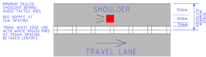
Figure 5.2.1.2 Retrofit ATEL Installation - Absolute minimum sealed shoulder 0.35m with on-line audio tactile ribs
