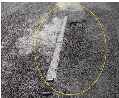
Photo 7.4. Plucking of audio tactile ribs on low texture seals
