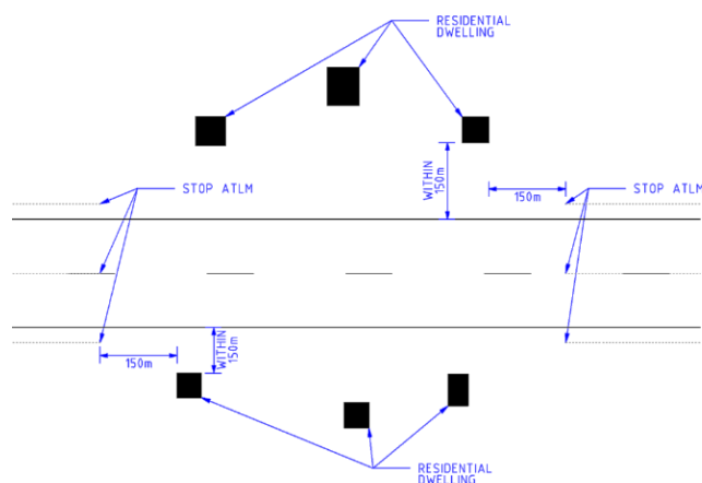
Figure 3.3 ATLM Installation where there is a cluster of residential properties
