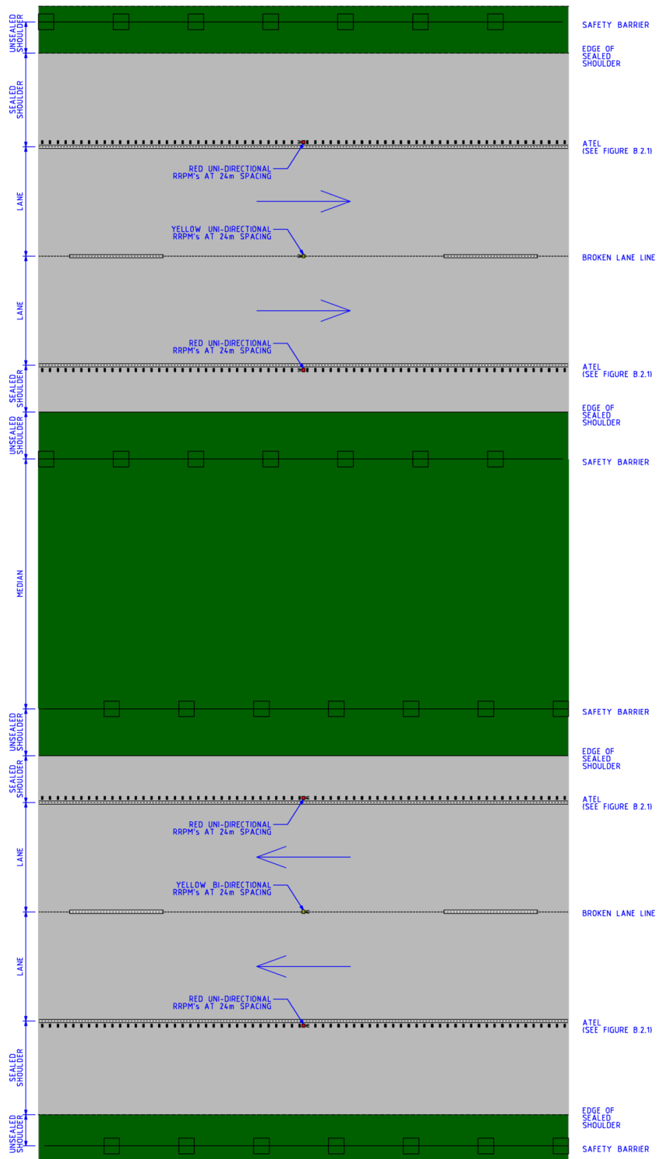
Figure C.4.1 – Plan Layout with Audio Tactile Line Marking (ATLM) and Divided Roads
