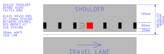
Figure 4.2.1 ATEL Installation - Absolute minimum sealed shoulder 0.5m
