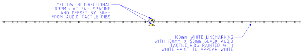
Figure B.1.2 – Single Two-Way Barrier ATCL
