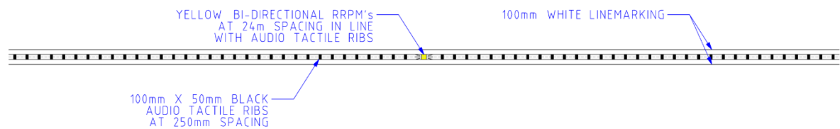
Figure B.1.3 – Double Two-Way Barrier ATCL
