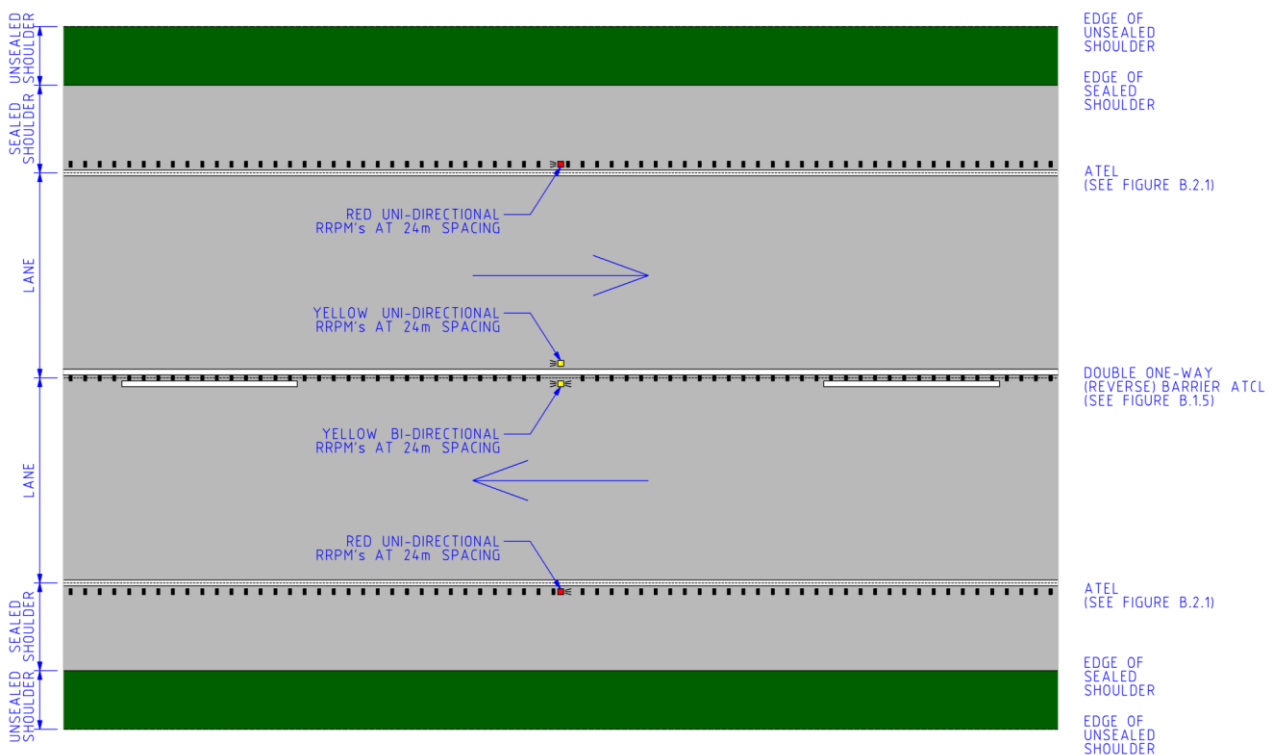
Figure C.2.4 – Plan Layout with Double One-Way Barrier (Reverse) ATCL and Audio Tactile Edge Line (ATEL)
