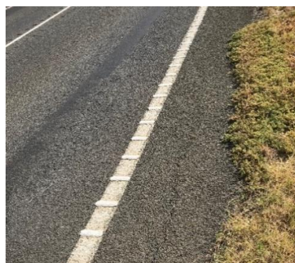
Photo 5.2.1.1 ATEL with on-line painted black ribs
