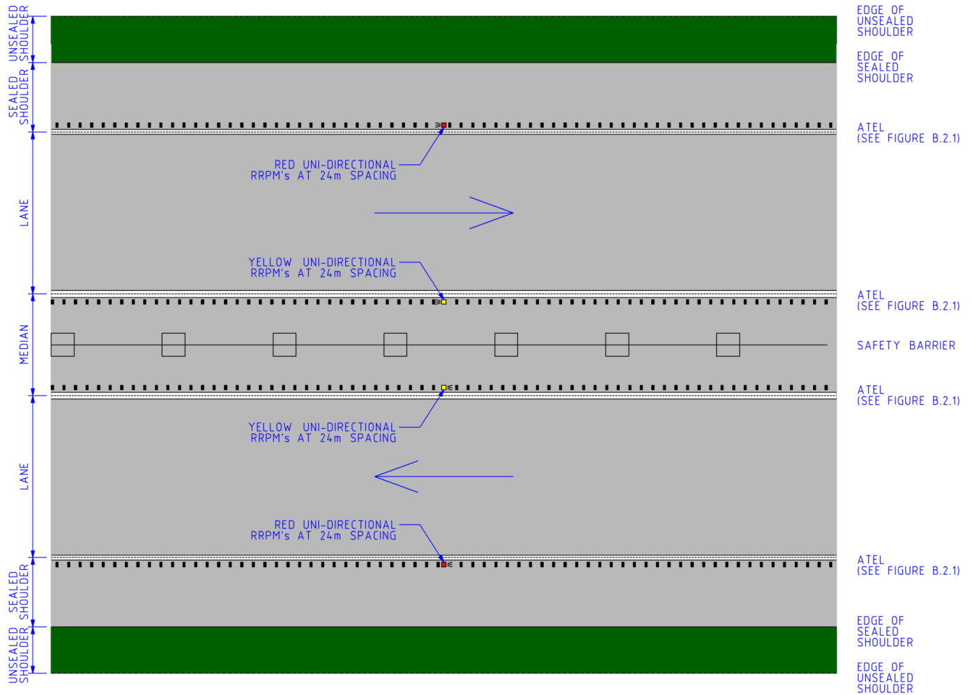
Figure C.3.1 – Plan Layout with Audio Tactile Line Marking (ATLM) and Central Barrier in Narrow Medians
