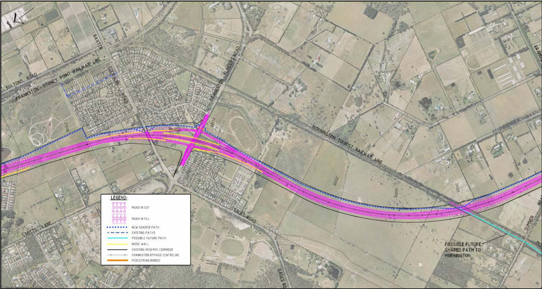
Figure 5.1 Frankston Bypass proposed concept layout (Sheet 5 of 8)
