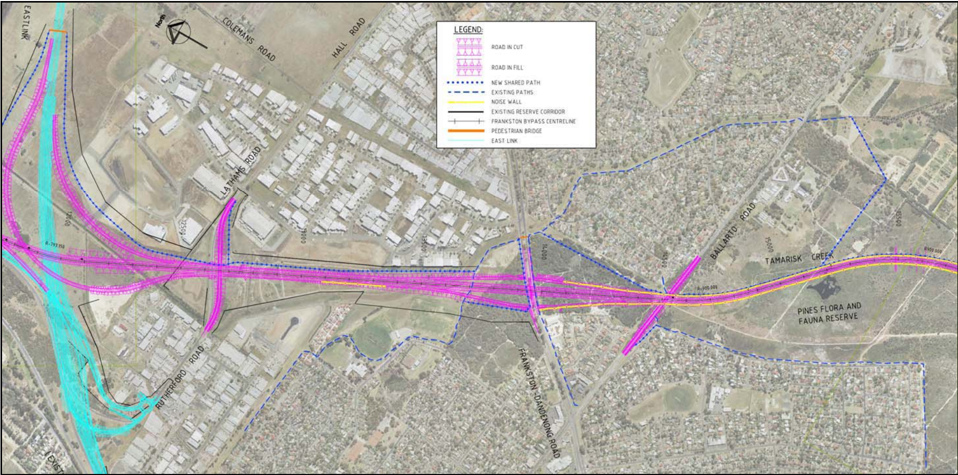
Figure 5.1 Frankston Bypass proposed concept layout (Sheet 2 of 8)
