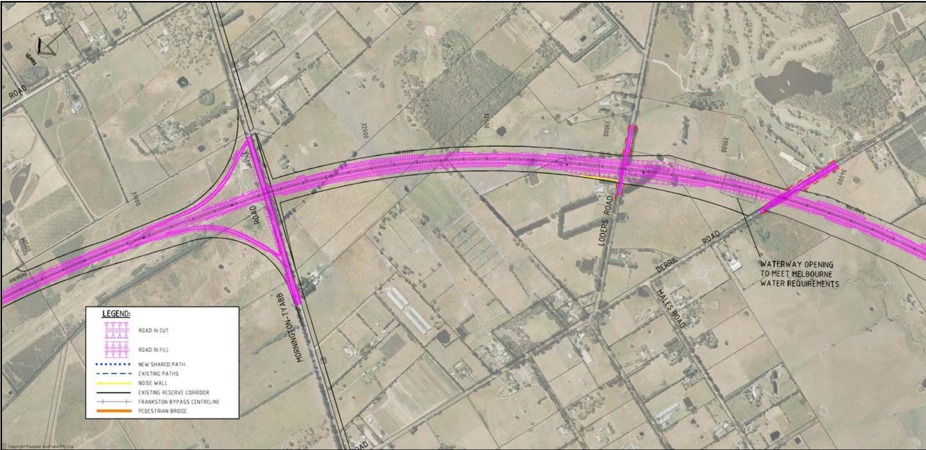
Figure 5.1 Frankston Bypass proposed concept layout (Sheet 7 of 8)
