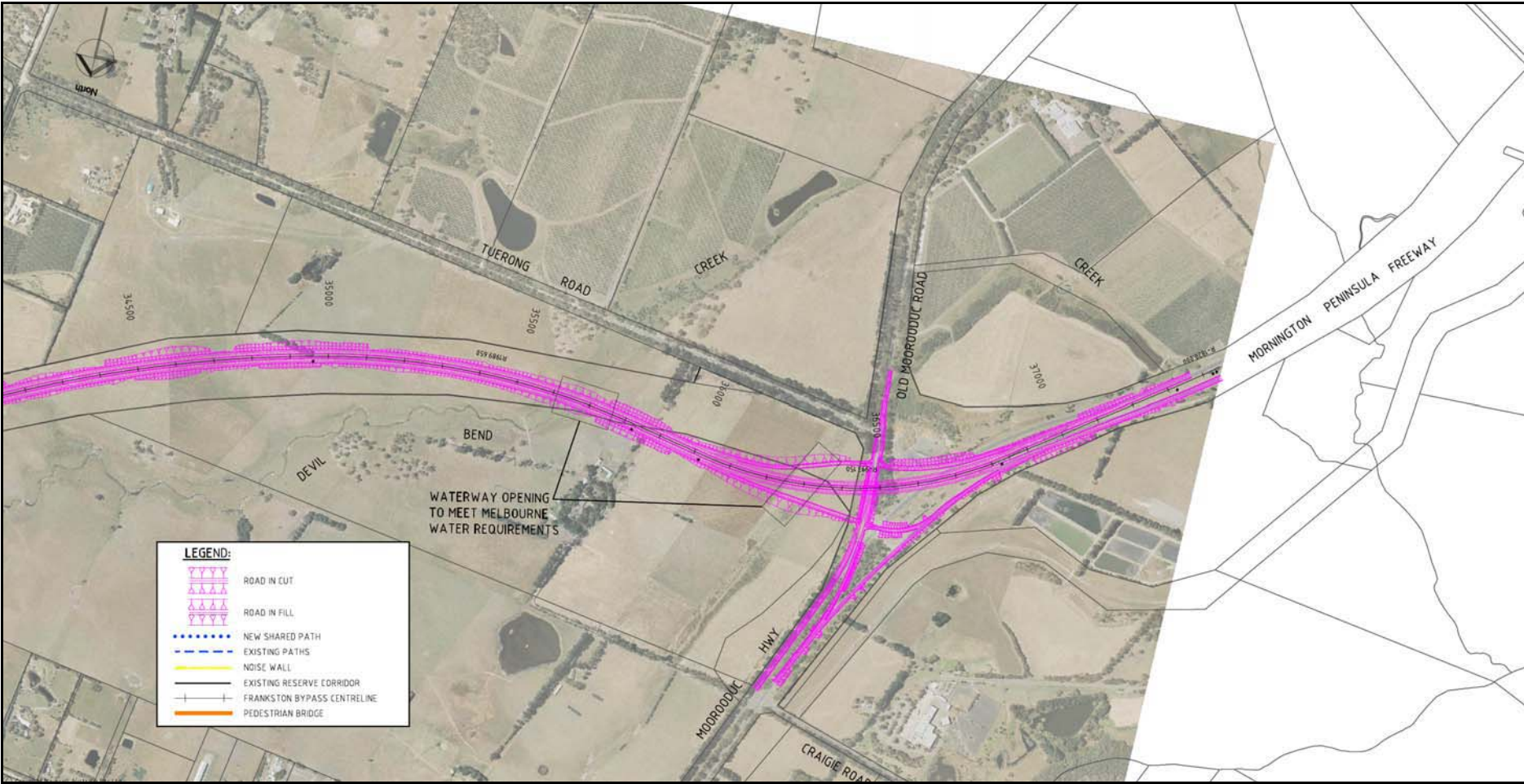
Figure 5.1 Frankston Bypass proposed concept layout (Sheet 8 of 8)
