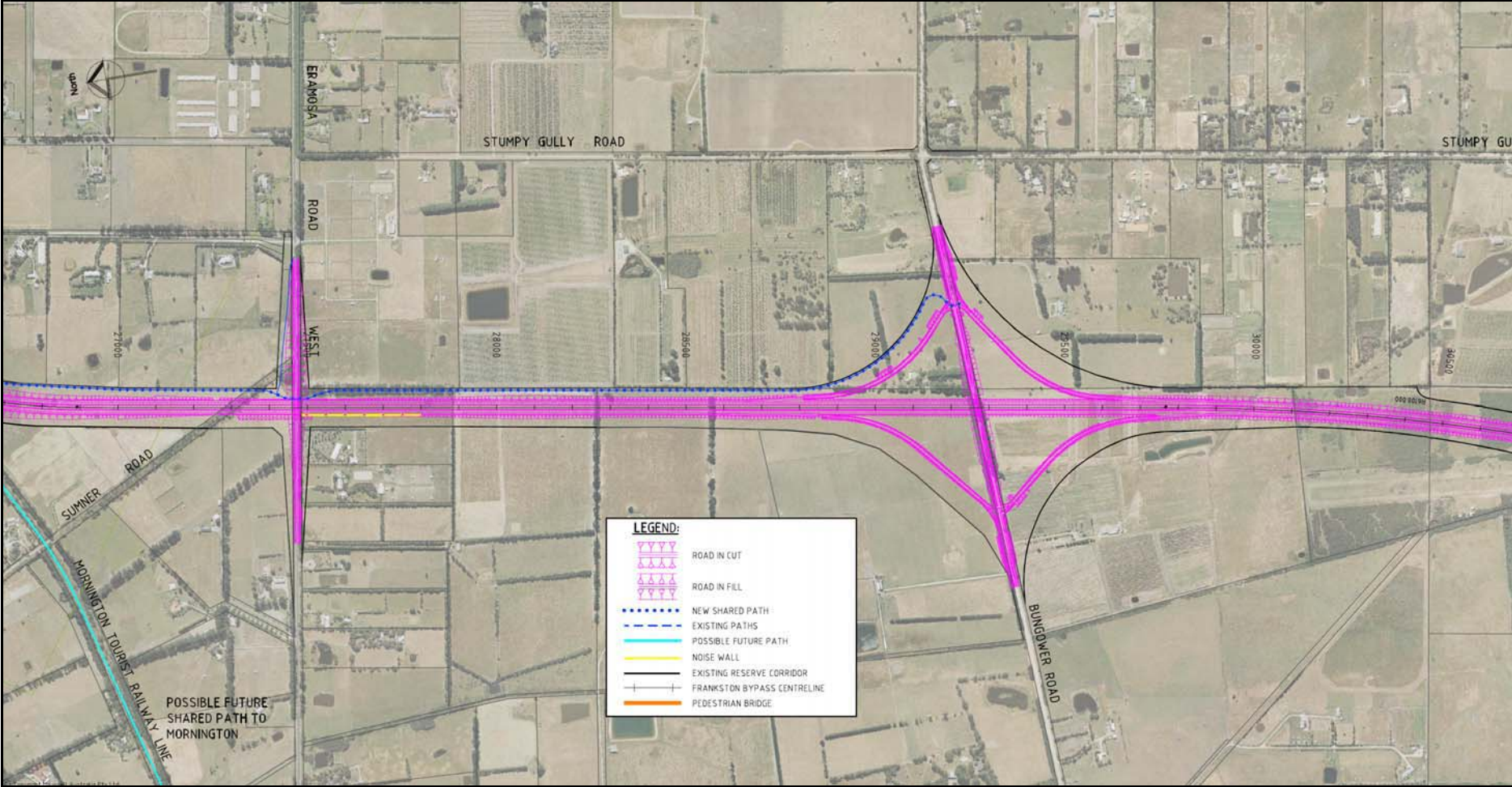
Figure 5.1 Frankston Bypass proposed concept layout (Sheet 6 of 8)
