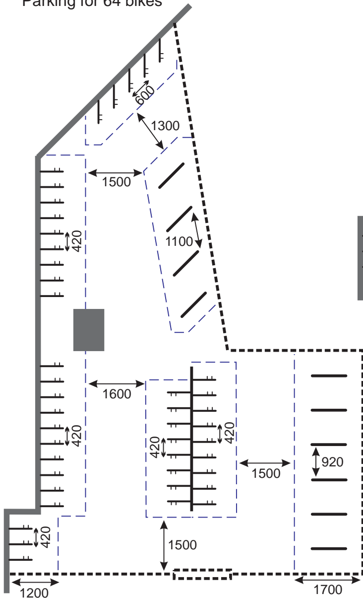
Figure 3 Parking for 64 bikes
