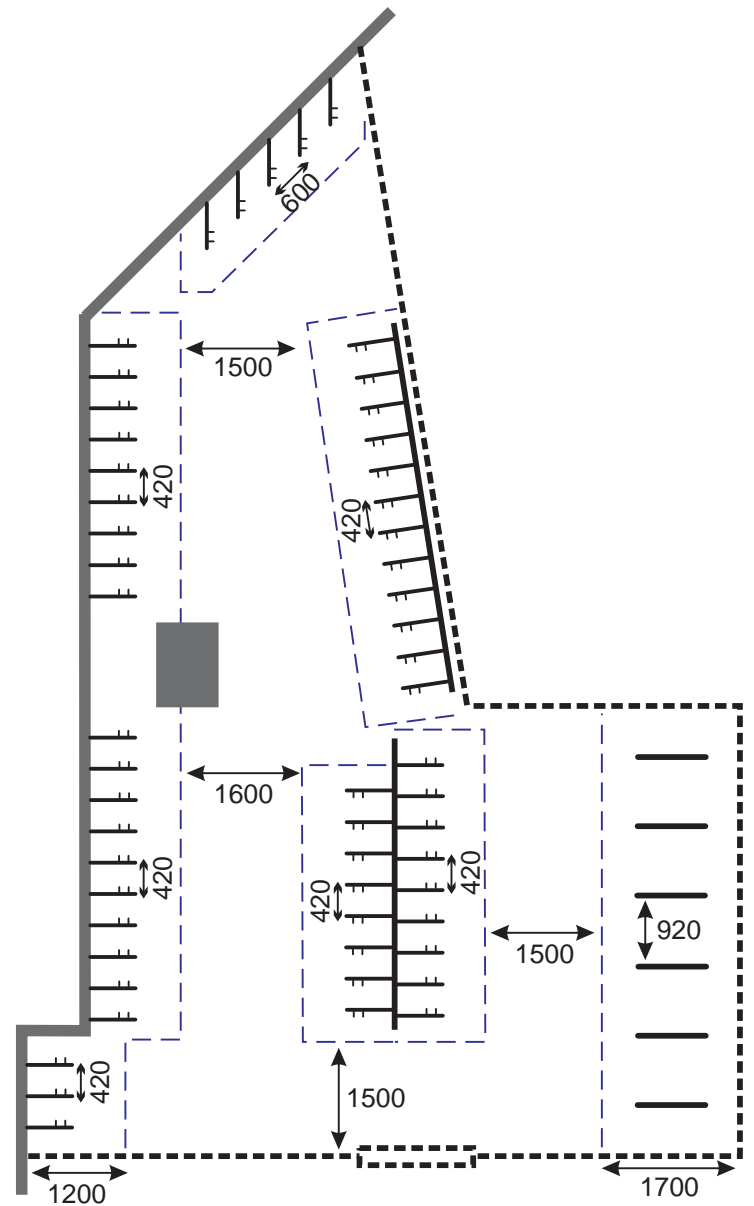
Figure 4 Parking for 68 bikes
